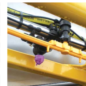
Dual nozzle bodies fitted to twin fold boom
