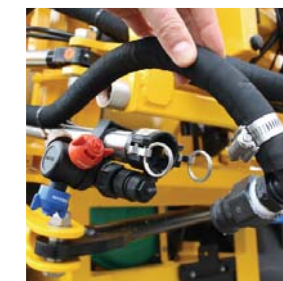
Spray line quick release drain point
